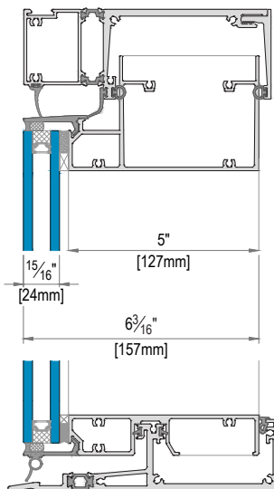
TYPICAL RWW 9000 SERIES SECTION DETAIL
