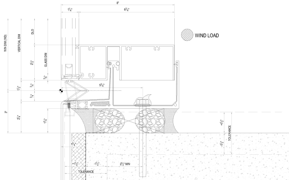
15 TYPICAL SILL - WIND LOAD DETAIL
