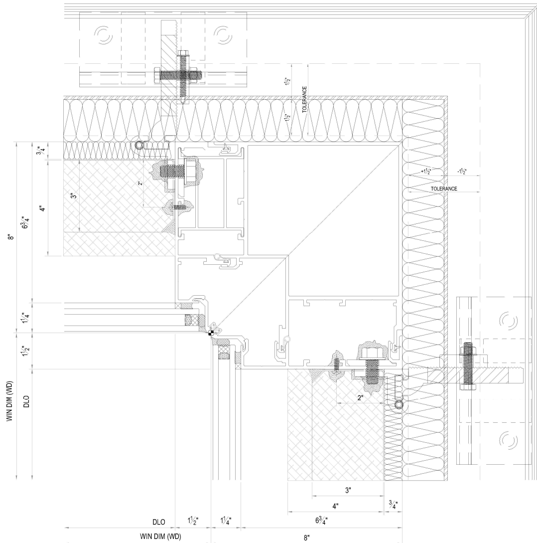
31 90° TYPICAL INSIDE CORNER ANCHOR DETAIL
