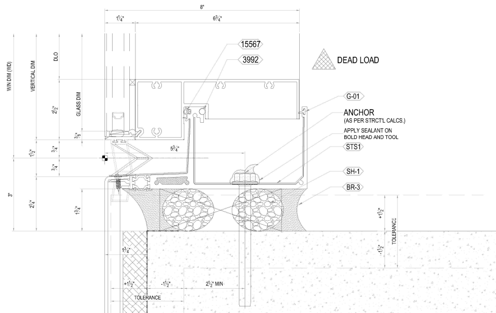
16 TYPICAL SILL - DEAD LOAD DETAIL
