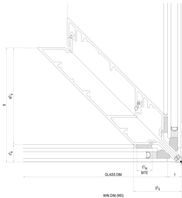
25 TYPICAL 90° OUTSIDE CORNER DETAIL
