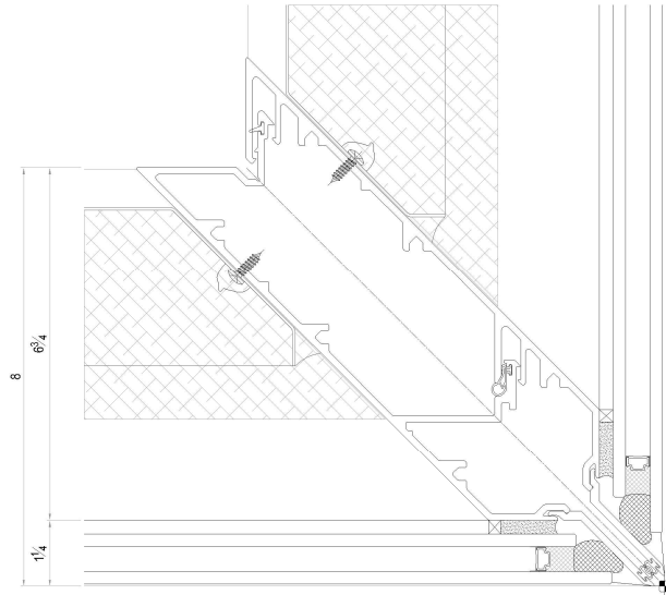
26 90° OUTSIDE CORNER SPANDREL DETAIL
