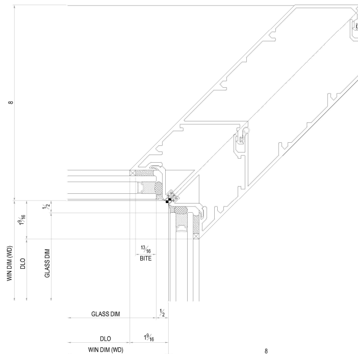
32 90° TYPICAL INSIDE CORNER DETAIL
