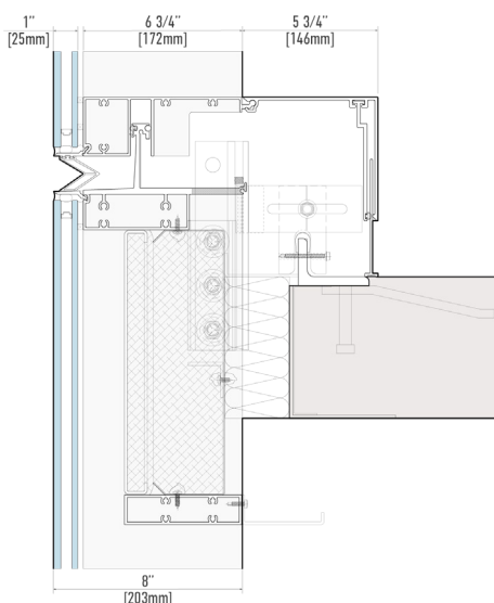
TYPICAL RWW 8000 SERIES SECTION DETAIL
