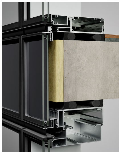
RWW 12000 SERIES SECTION VIEW
