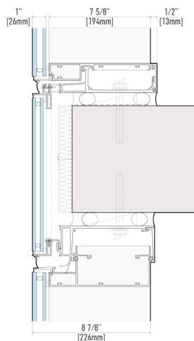
TYPICAL RWW 12000 SERIES SECTION DETAIL
