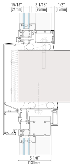
TYPICAL RWW 7000 SERIES SECTION DETAIL
