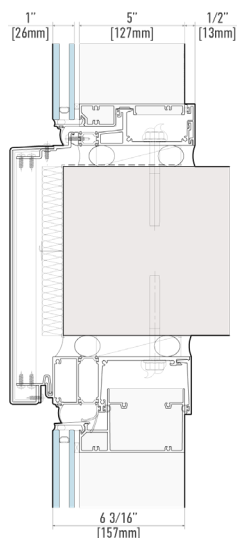
TYPICAL RWW 9000 SERIES SECTION DETAIL
