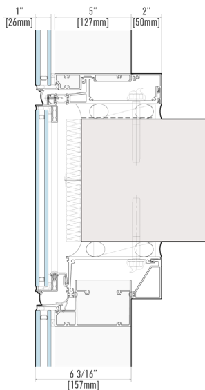
TYPICAL RWW 9500 SERIES SECTION DETAIL
